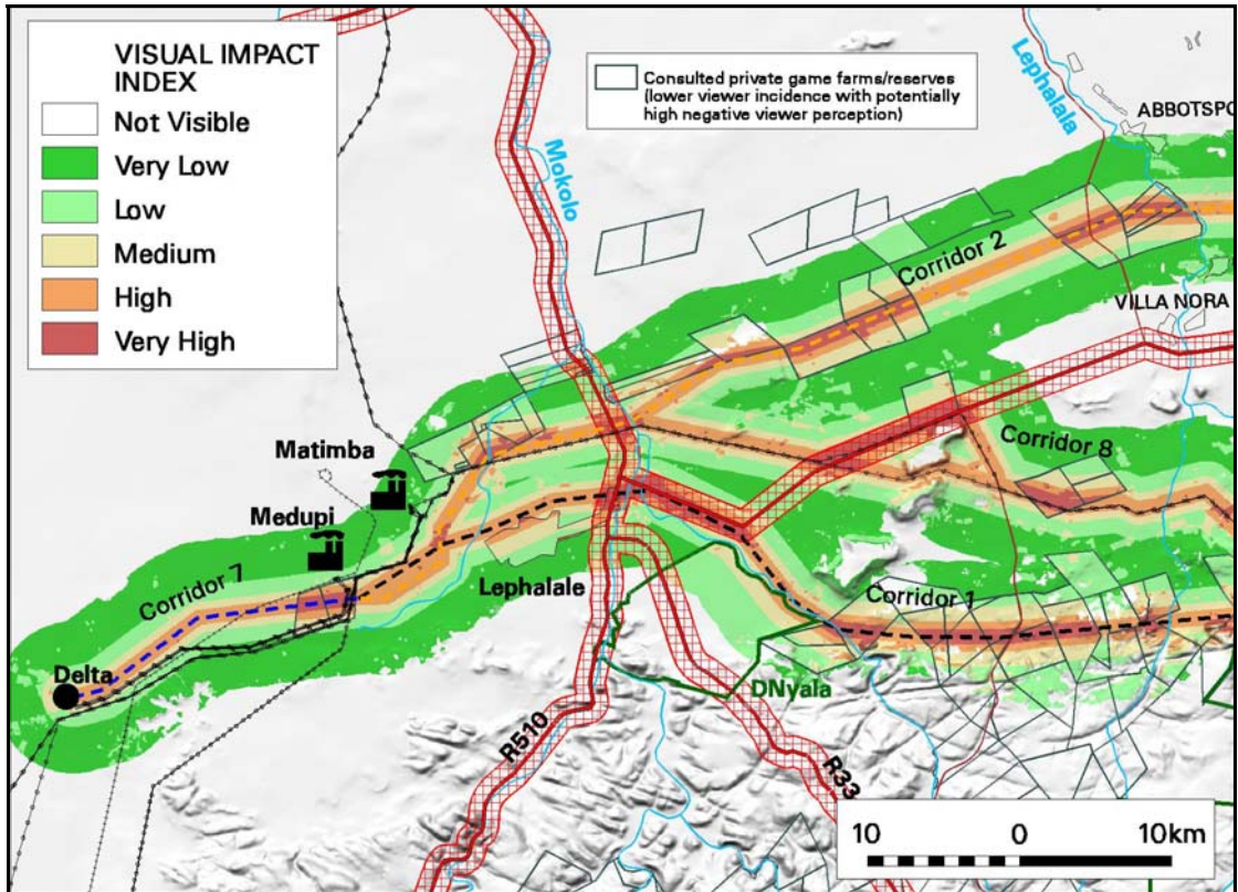
Figure 21: Visual impact index - transmission line Alternatives 1, 2, 7 and 8 (western section).
