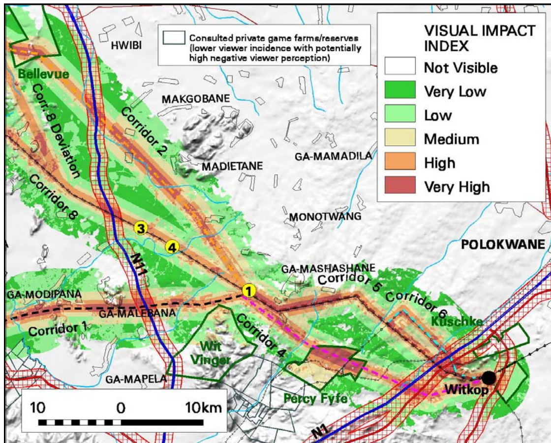
Figure 23: Visual impact index - transmission line Alternatives 1, 2, 4, 5, 6, 8 and 8a (eastern section).
